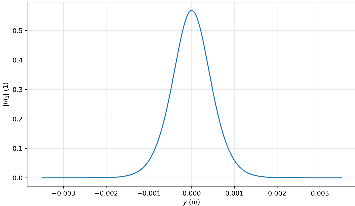
Intensity profile I(x=0, y, z=3.503)/I_0 , P_{in}=0.6P_{cr} , artificial time
